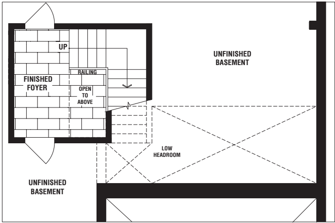
PARTIAL BASEMENT PLAN W/ OPT. GROUND FLOOR ELEV. 'A' & 'B' (ELEV. 'C' SIMILAR)
